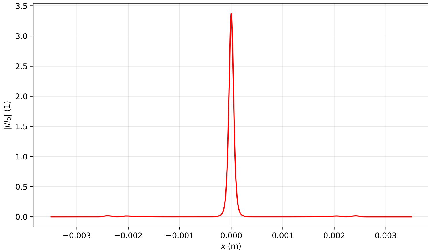
Intensity profile I(x, y = 0, z = 2.388)/I_0 , P_{in}=9.0P_{cr} , artificial time
